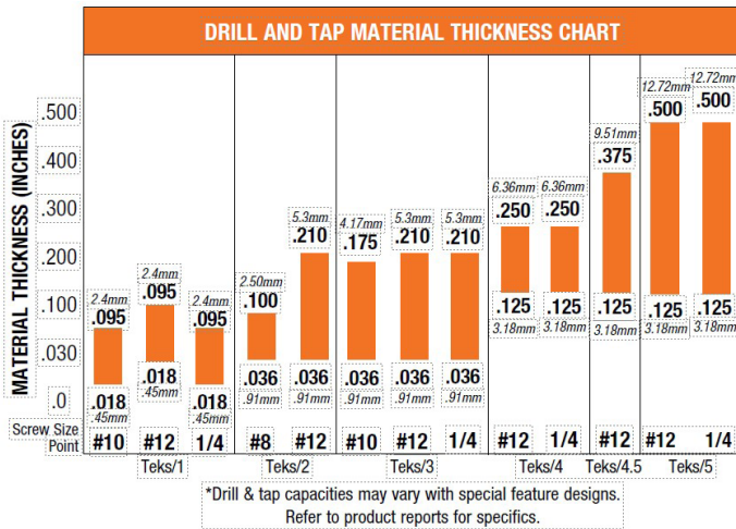
Drilling and Tapping Capacity (Maximum Material Thickness)
