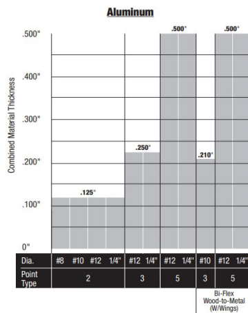
Drilling and Tapping Capacity (Maximum Material Thickness)
