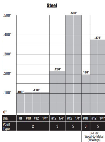
Drilling and Tapping Capacity (Maximum Material Thickness)
