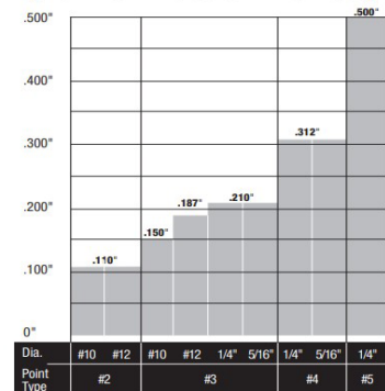
Drilling and Tapping Capacity (Maximum Material Thickness)*
